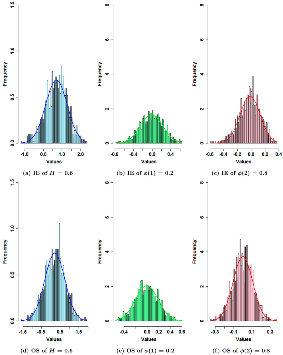
Figure 6. The simulation of initial estimator and one-step estimator where \theta = (0.2, 0.8, 0.6) for m = [n^{1/3}], n = 2000 .
