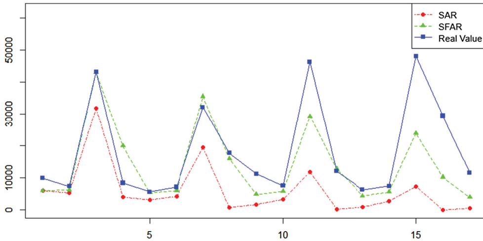
Figure 9. Model fitting plot.
