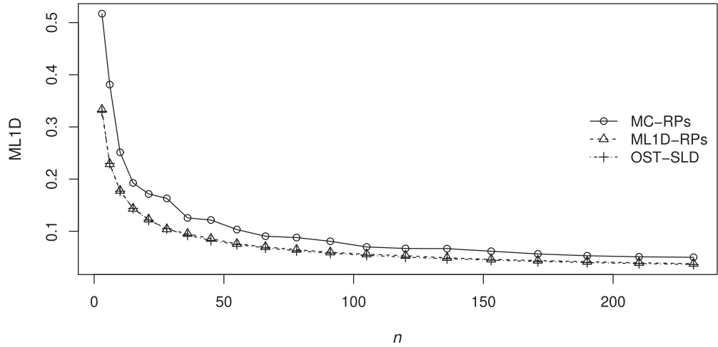
Figure A5. Mean L_1 -distance (ML1D) criterion values for MC-RPs, ML1D-RPs, OST-SLD as n increases ( n = \binom{p+m-1}{m}, m = 1, \dots, 20, p = 3 ).
